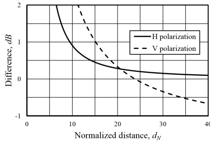
Fig. 5. Dependence of the field strength difference between calculated in line with Vvedenskij's formula and exact equations [2] on normalized distance ( h=3 m, f=100 MHz).
