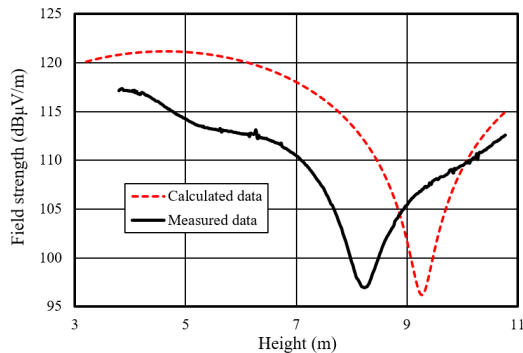
Fig. 3. The field strength level as a function of the height ( f = 96.3 MHz, P = 29.7 dBW, H = 60 m, d = 346 m).
