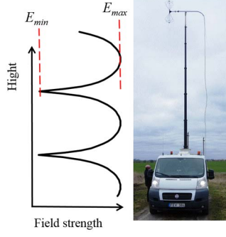
Fig. 1. The dependency of the field strength on height.
