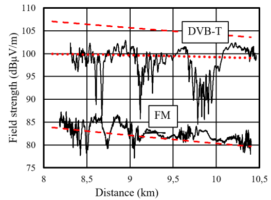
Fig. 7. The field strength level as a function of the distance from the transmitting antenna along the route J1. – measured data; - - -, ••• calculated data according two-ray and free-space models respectively.
