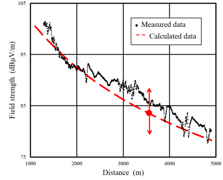
Fig. 4. The field strength level as a function of the distance from the transmitting antenna along a route which coincides with antenna's beam axis.
