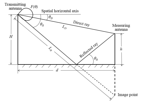
Fig. 2. Geometry of the two-ray ground reflected model.
